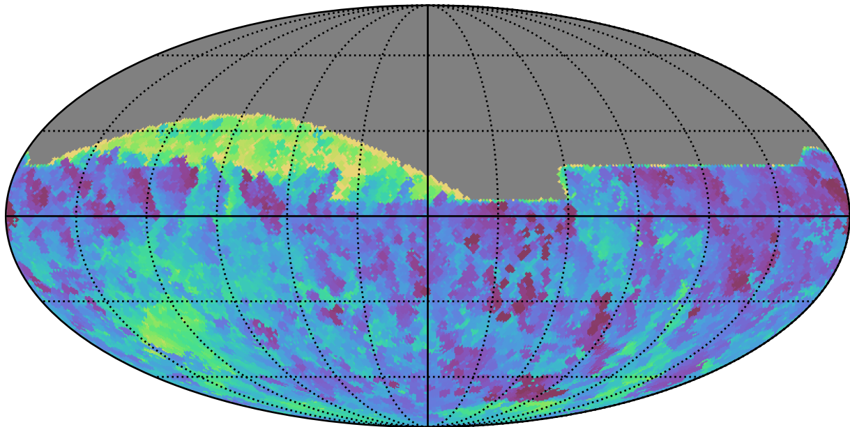
baseline_v3.5_10yrs All sky all bands: Min fiveSigmaDepth
