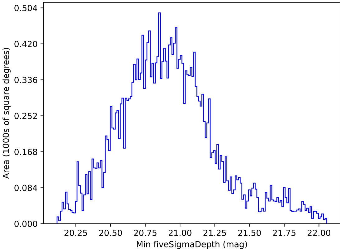
baseline_v3.5_10yrs All sky all bands: Min fiveSigmaDepth
