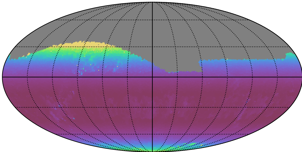
baseline_v3.5_10yrs Yr 1 z band: Min airmass
