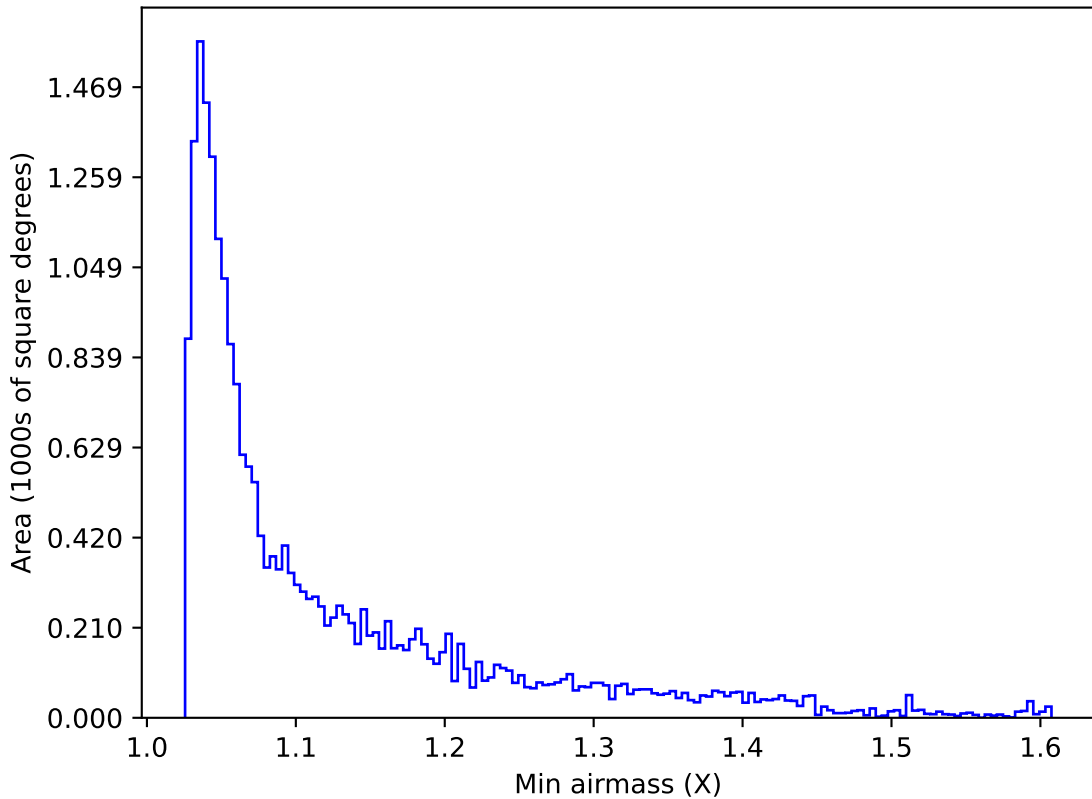
baseline_v3.5_10yrs Yr 1 y band: Min airmass
