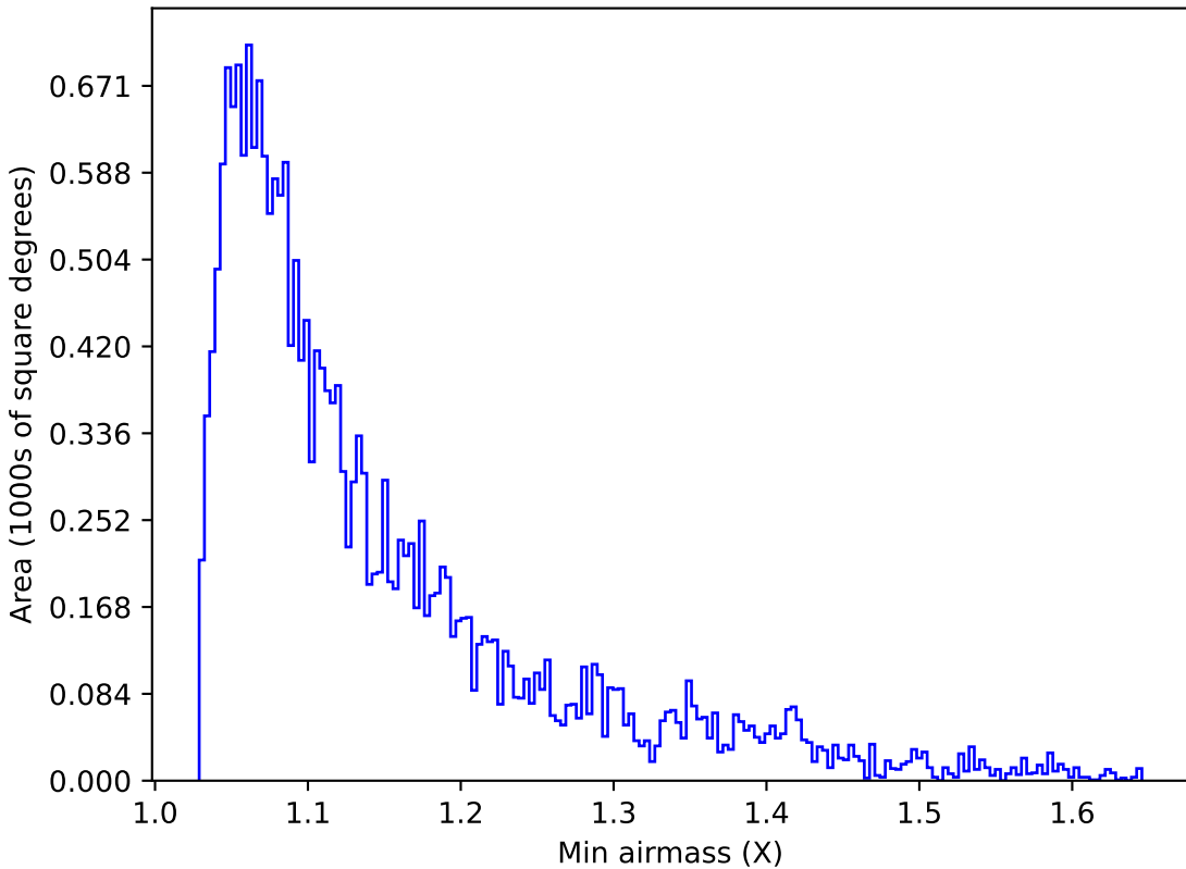
baseline_v3.5_10yrs Yr 1 u band: Min airmass
