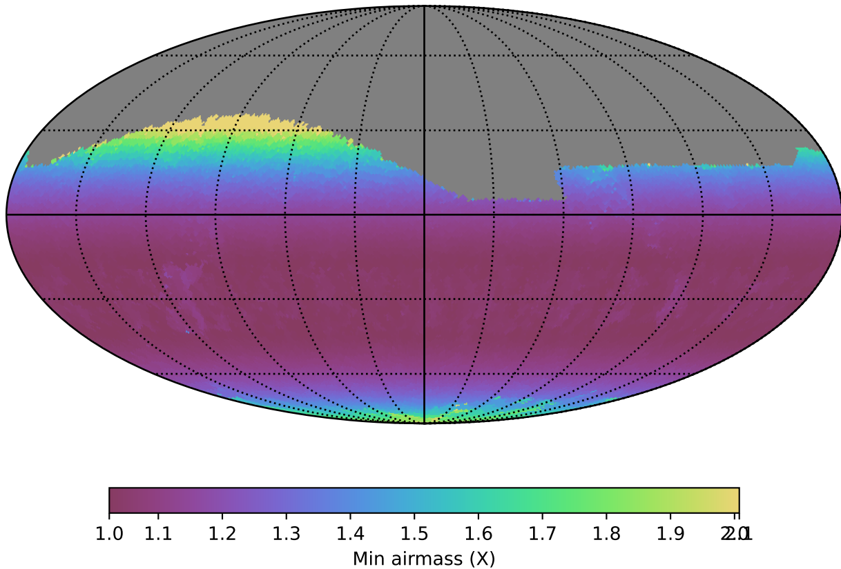
baseline_v3.5_10yrs Yr 1 r band: Min airmass
