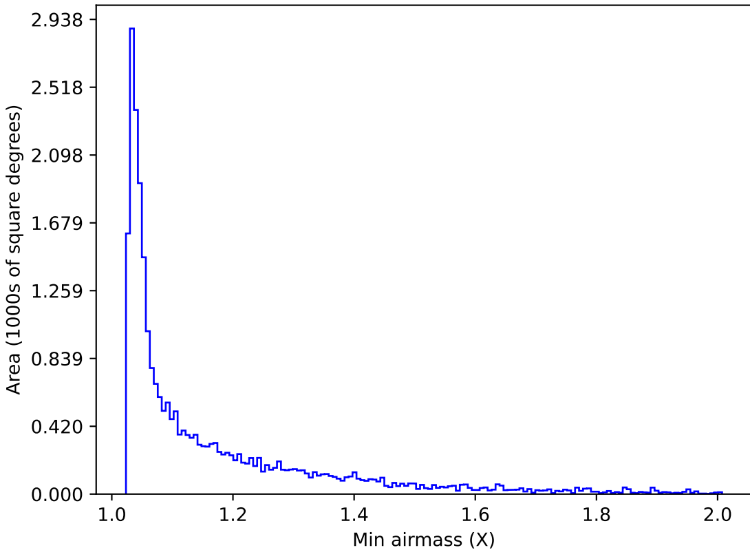
baseline_v3.5_10yrs Yr 1 r band: Min airmass
