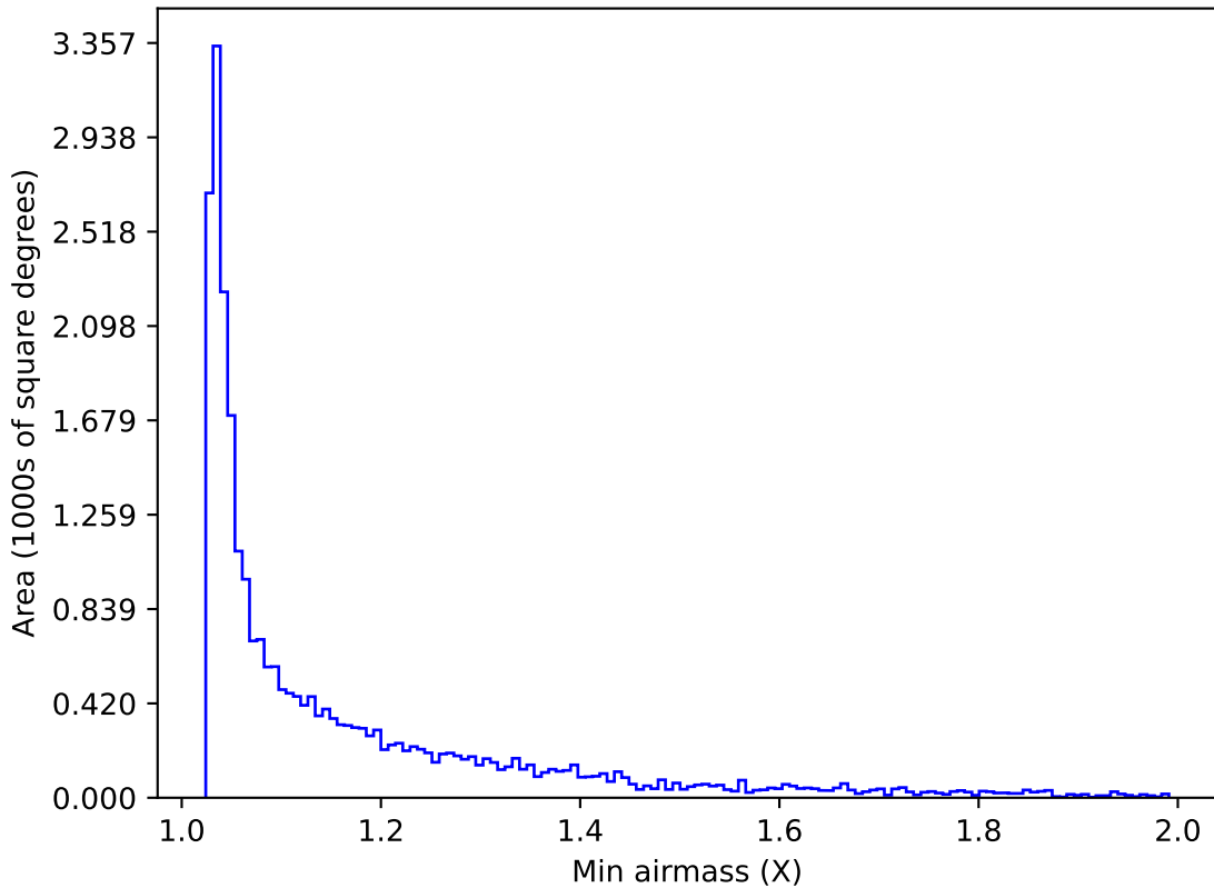
baseline_v3.5_10yrs Yr 1 i band: Min airmass
