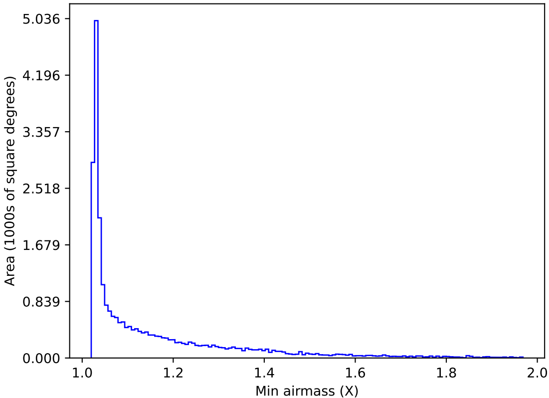
baseline_v3.5_10yrs Yr 1 all bands: Min airmass
