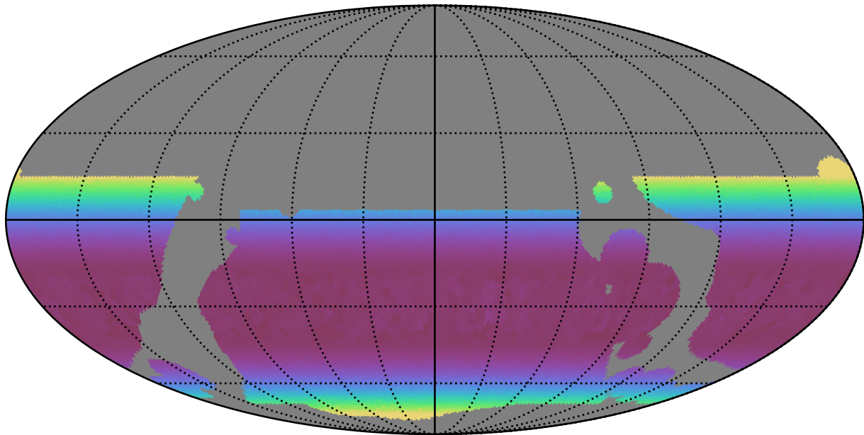
baseline_v3.5_10yrs WFD z band: Min airmass
