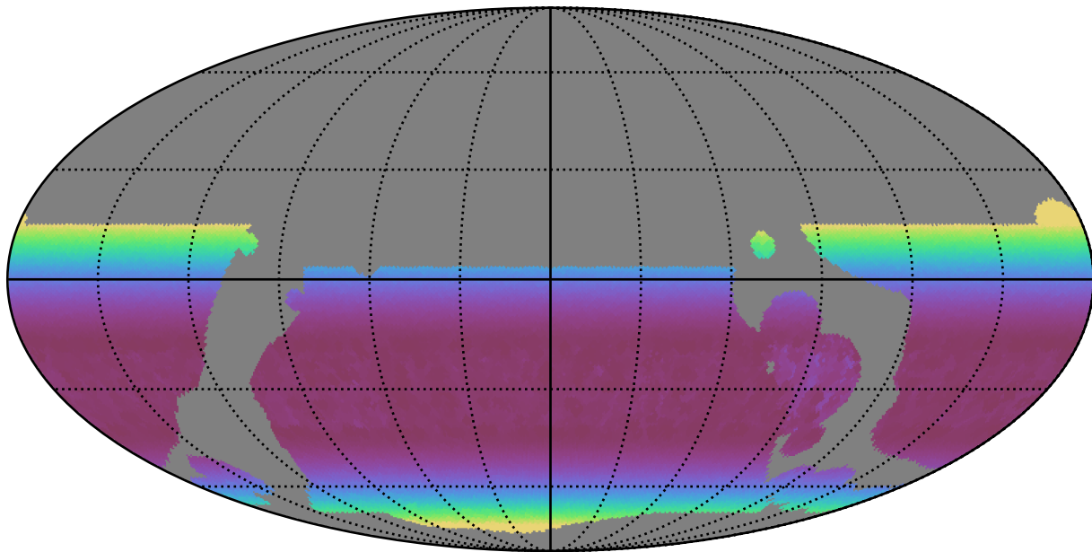
baseline_v3.5_10yrs WFD y band: Min airmass
