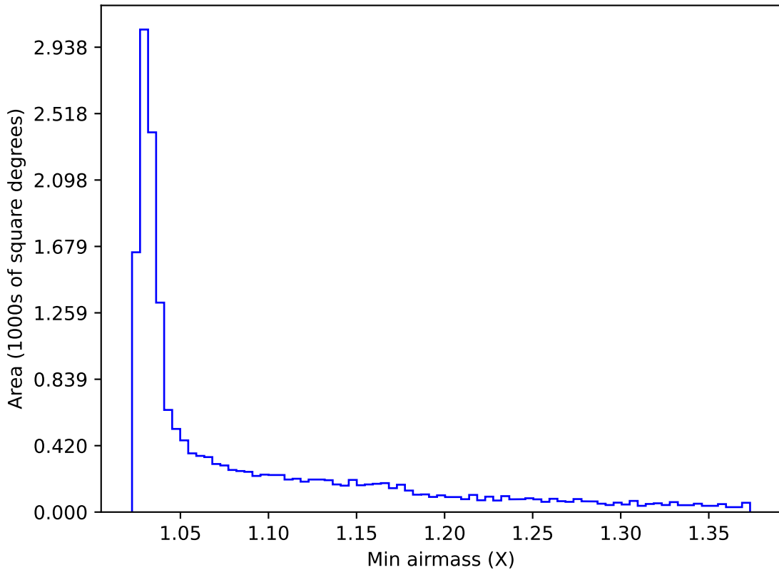
baseline_v3.5_10yrs WFD y band: Min airmass
