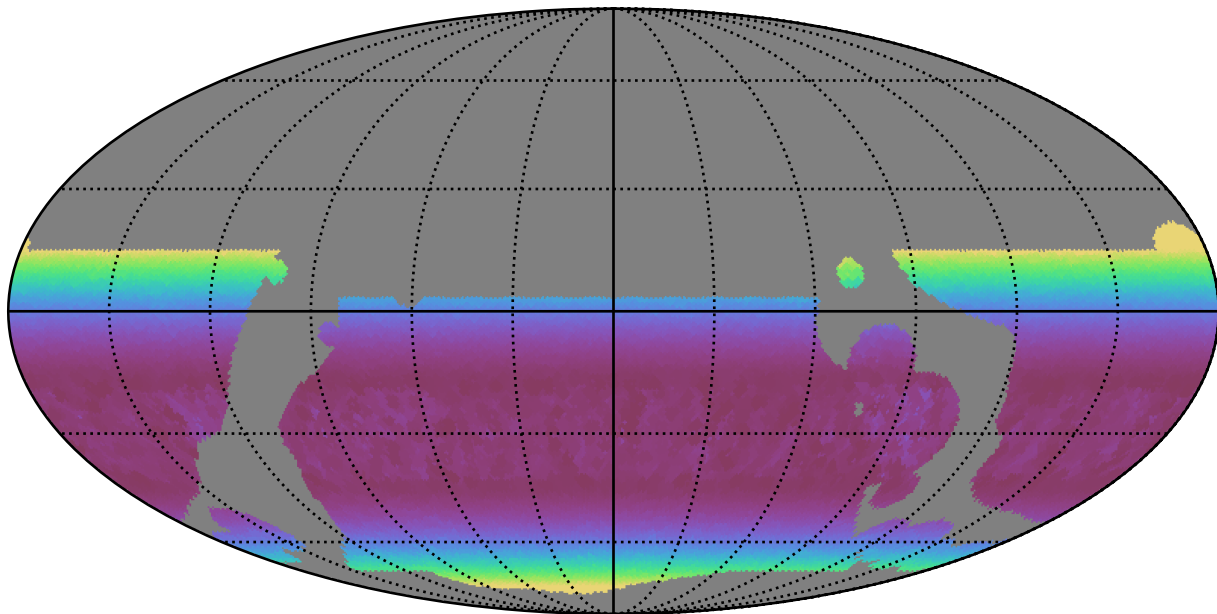
baseline_v3.5_10yrs WFD u band: Min airmass
