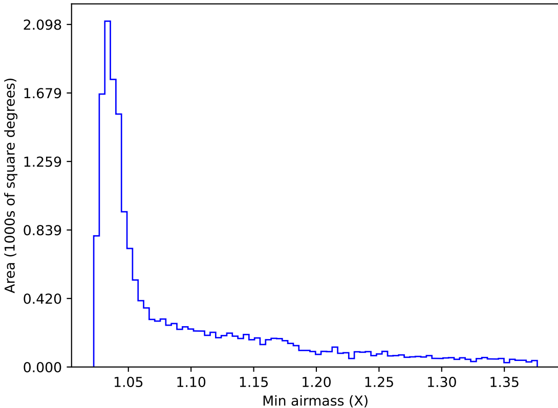
baseline_v3.5_10yrs WFD u band: Min airmass
