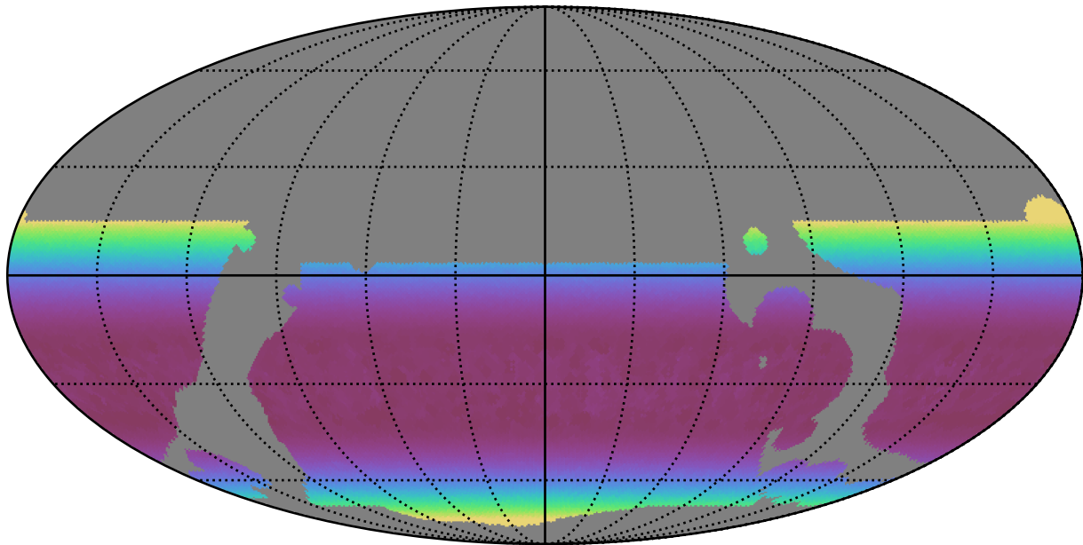
baseline_v3.5_10yrs WFD r band: Min airmass
