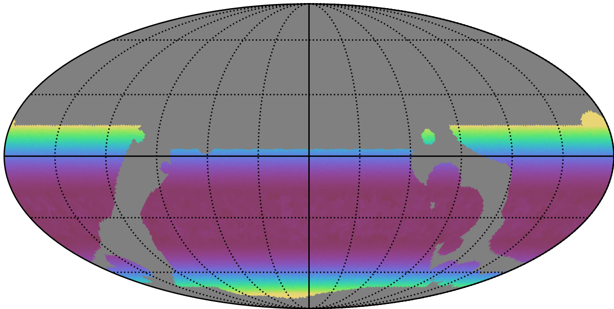
baseline_v3.5_10yrs WFD i band: Min airmass
