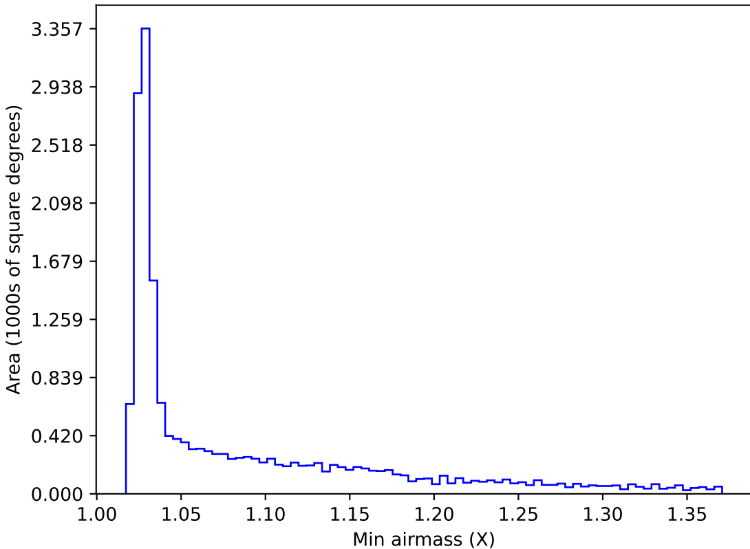
baseline_v3.5_10yrs WFD i band: Min airmass
