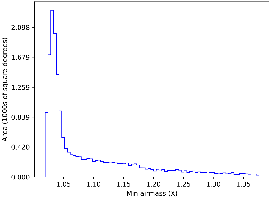
baseline_v3.5_10yrs WFD g band: Min airmass
