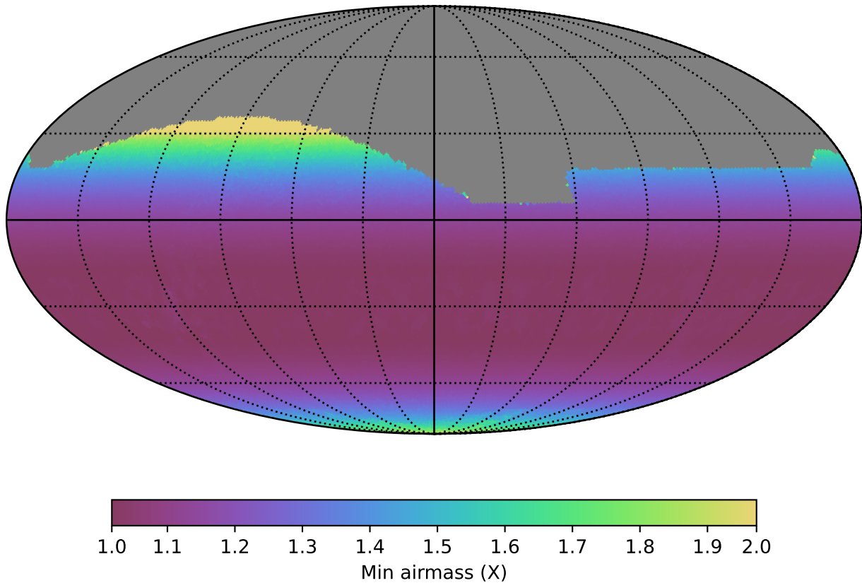
baseline_v3.5_10yrs All sky z band: Min airmass
