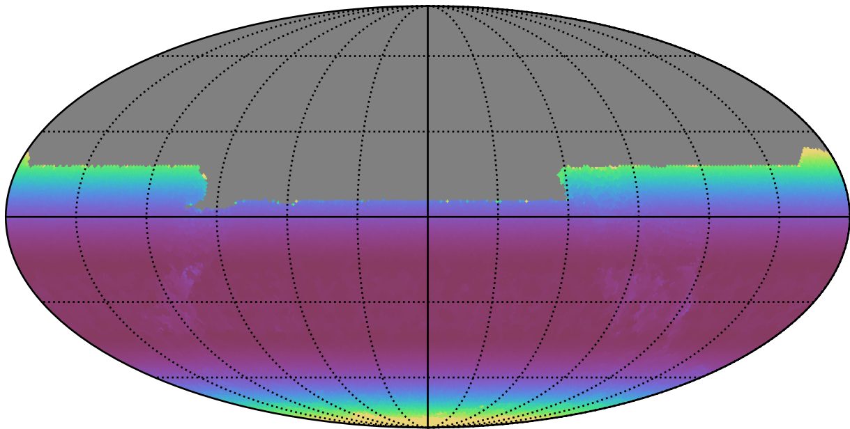
baseline_v3.5_10yrs All sky y band: Min airmass
