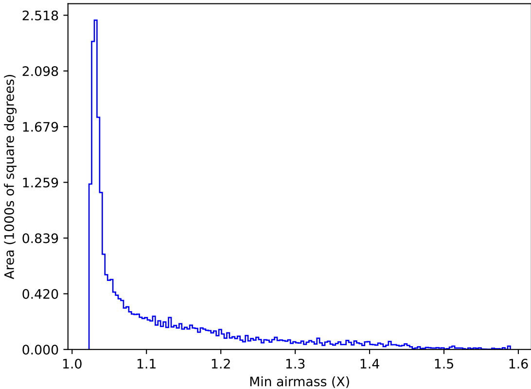
baseline_v3.5_10yrs All sky y band: Min airmass
