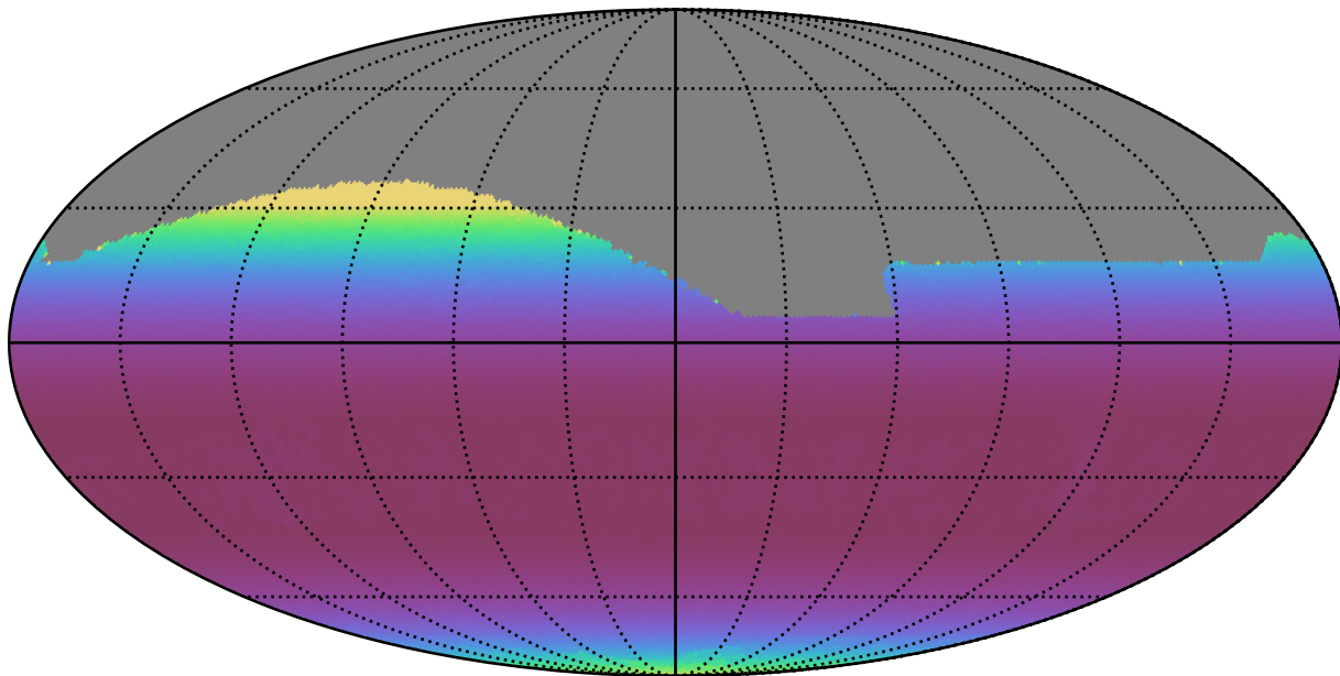
baseline_v3.5_10yrs All sky r band: Min airmass
