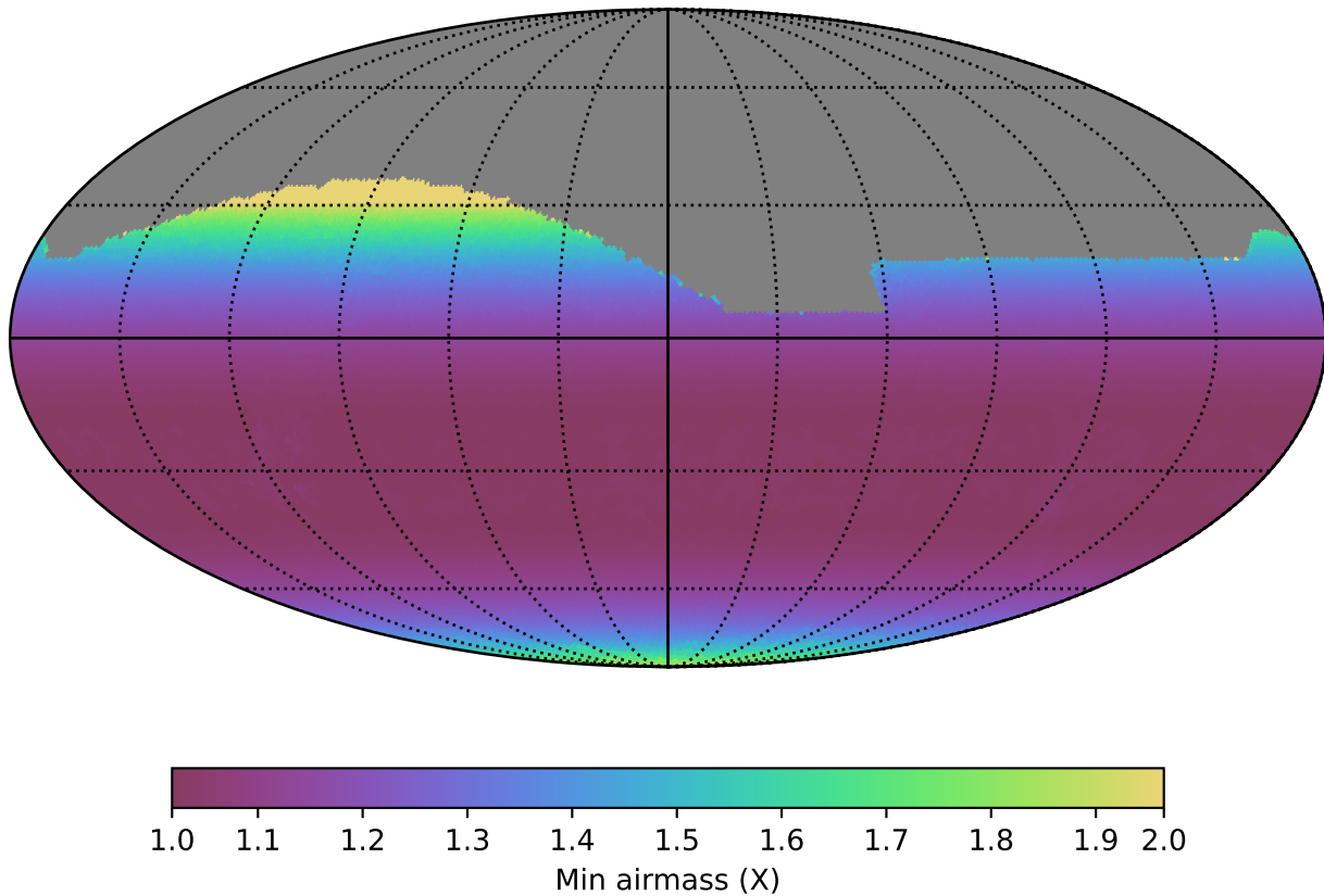
baseline_v3.5_10yrs All sky i band: Min airmass
