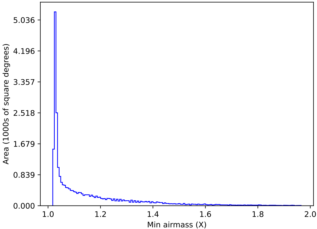
baseline_v3.5_10yrs All sky i band: Min airmass
