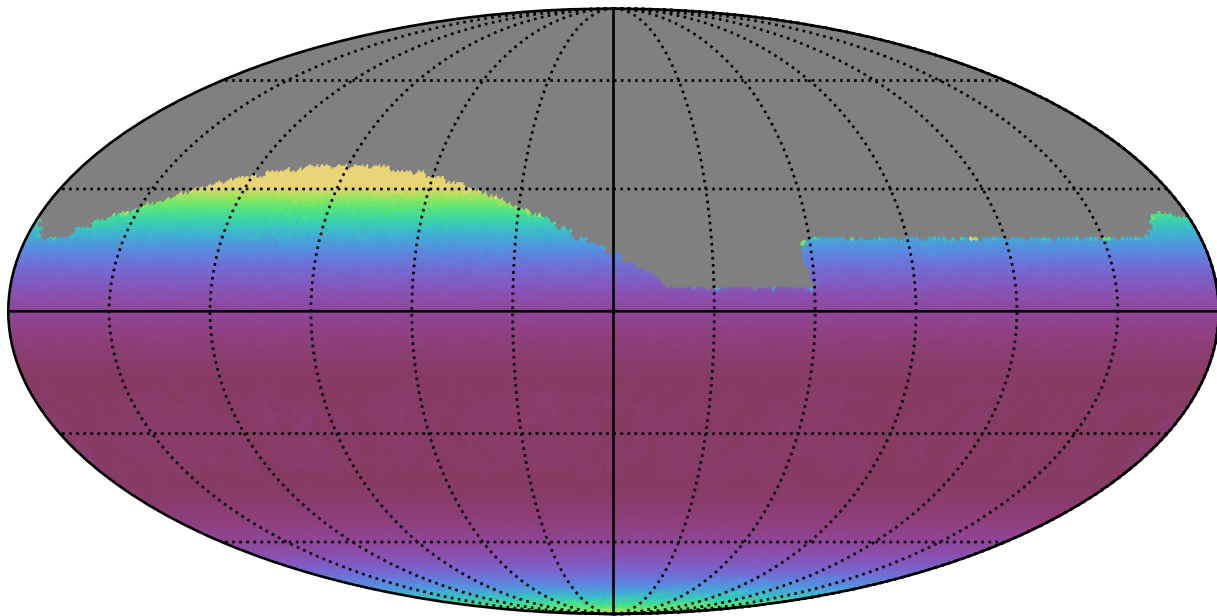
baseline_v3.5_10yrs All sky g band: Min airmass
