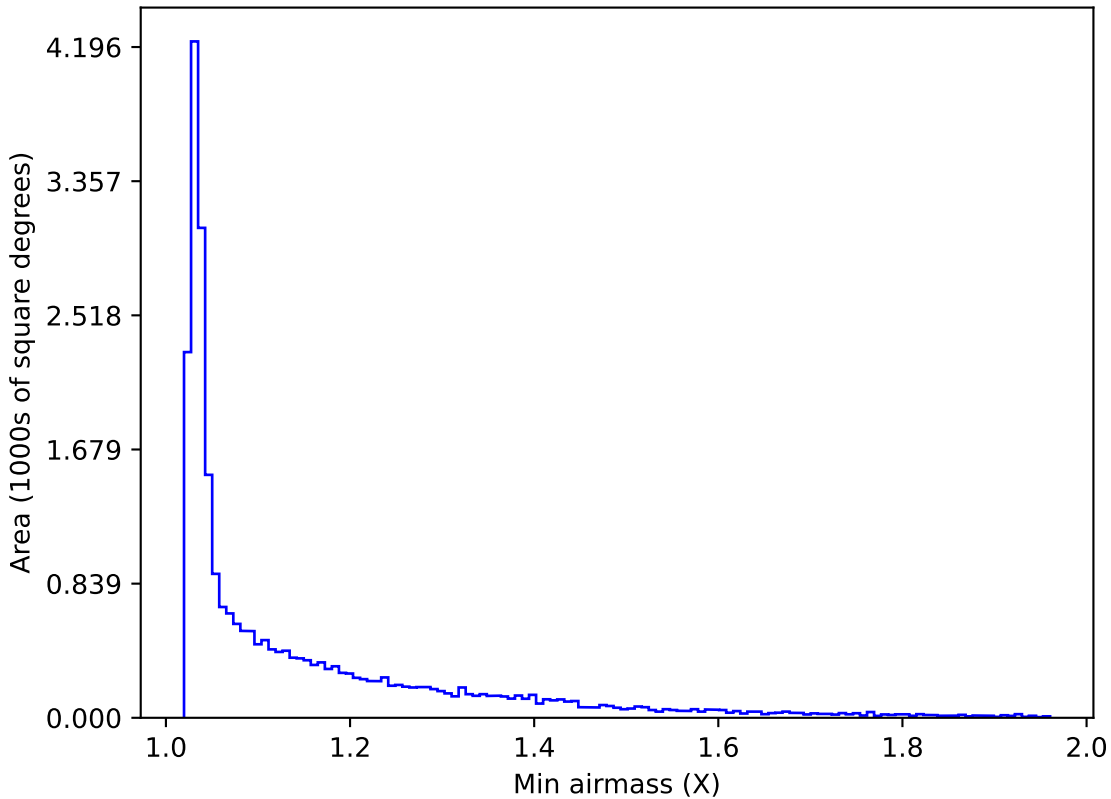
baseline_v3.5_10yrs All sky g band: Min airmass
