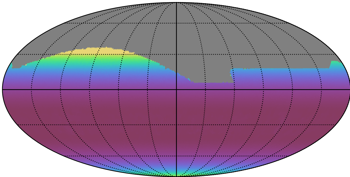
baseline_v3.5_10yrs All sky all bands: Min airmass
