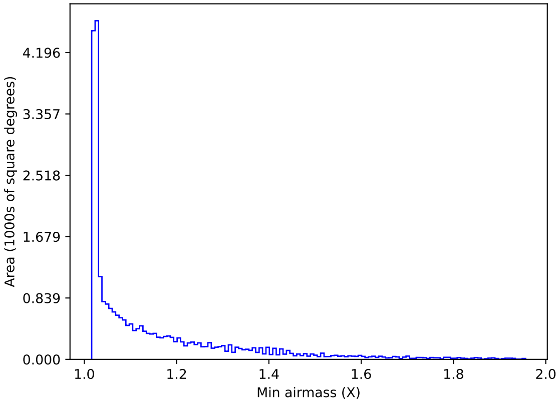
baseline_v3.5_10yrs All sky all bands: Min airmass
