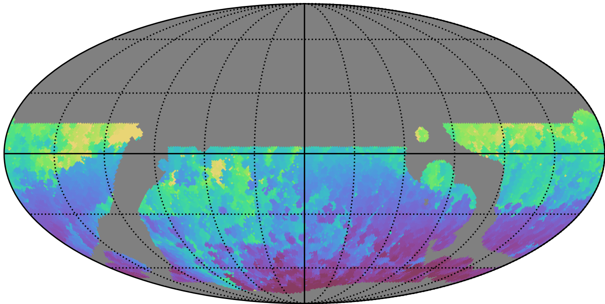
baseline_v3.5_10yrs WFD z band: Min HA
