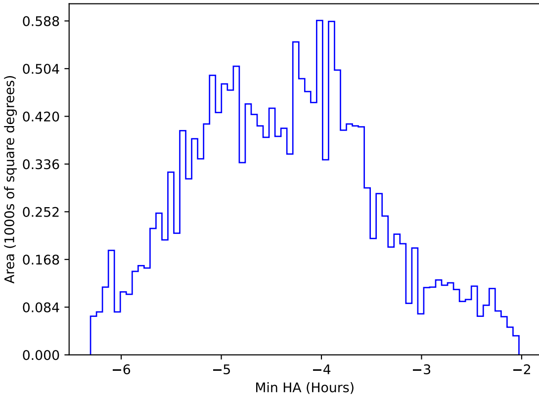
baseline_v3.5_10yrs WFD z band: Min HA
