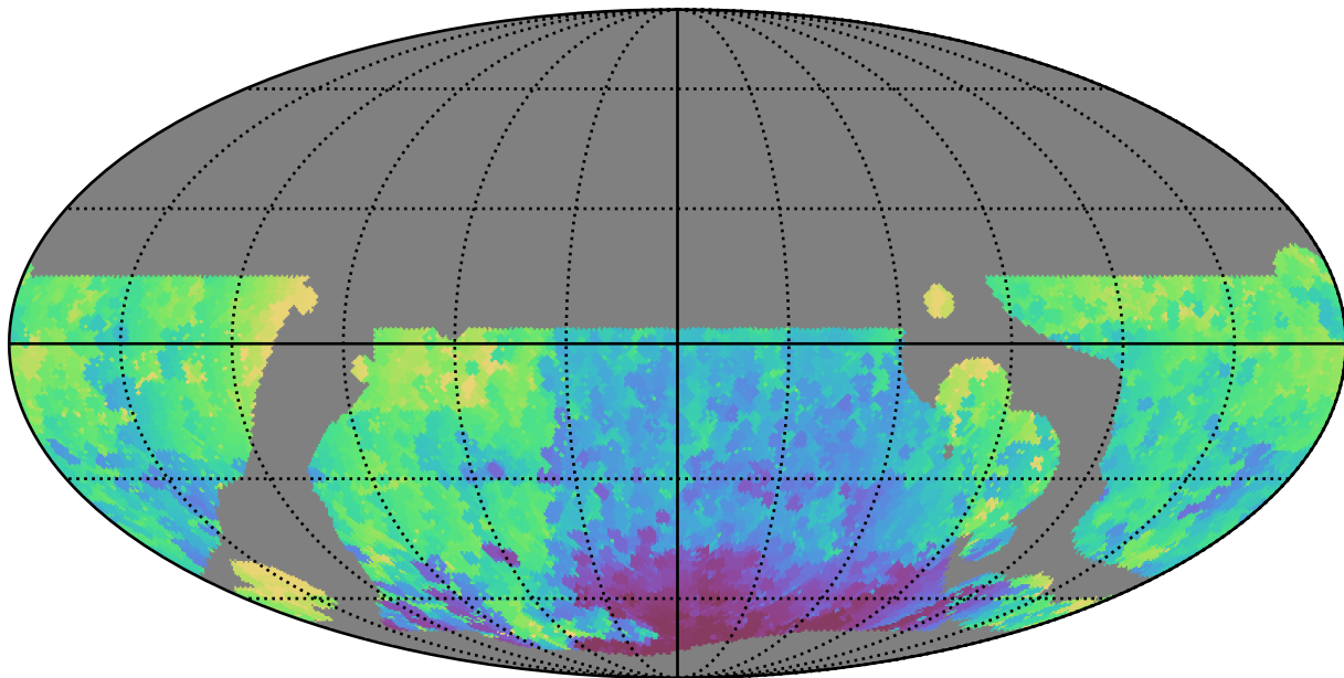
baseline_v3.5_10yrs WFD y band: Min HA
