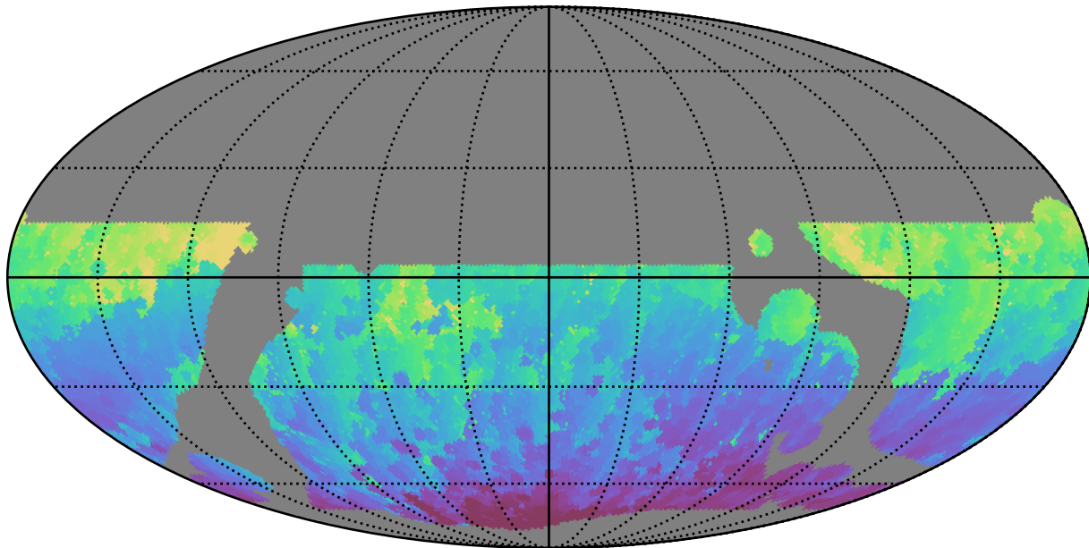
baseline_v3.5_10yrs WFD i band: Min HA
