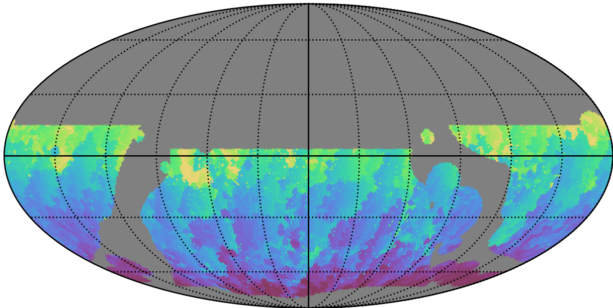
baseline_v3.5_10yrs WFD g band: Min HA
