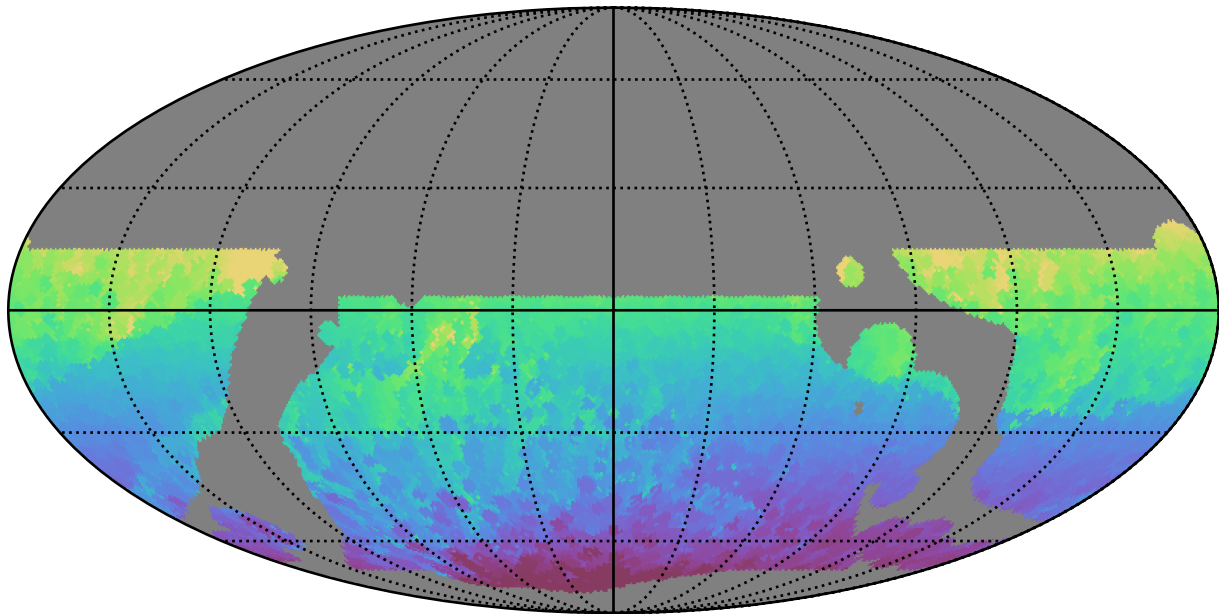
baseline_v3.5_10yrs WFD all bands: Min HA
