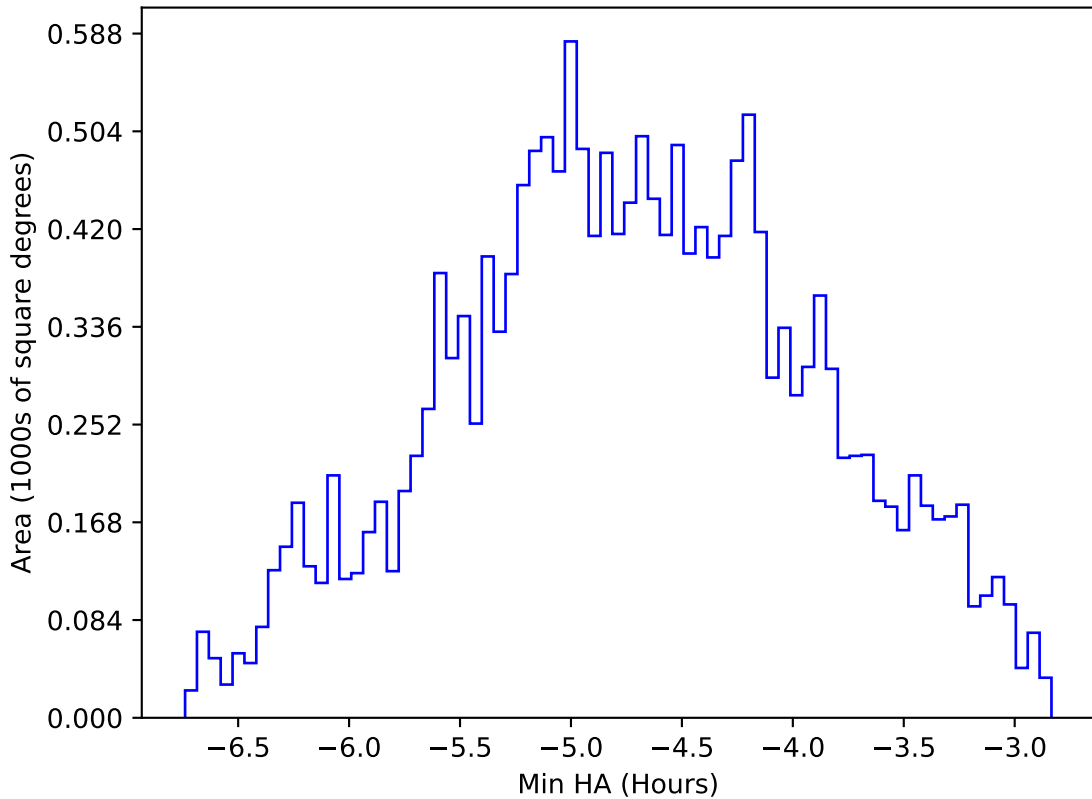
baseline_v3.5_10yrs WFD all bands: Min HA
