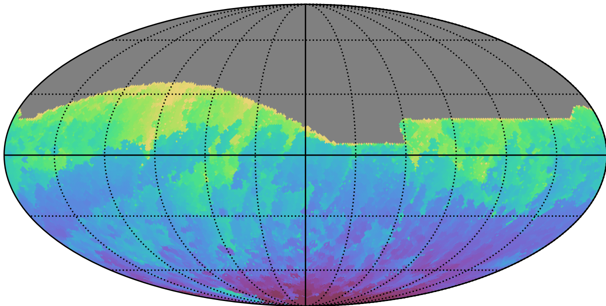
baseline_v3.5_10yrs All sky r band: Min HA
