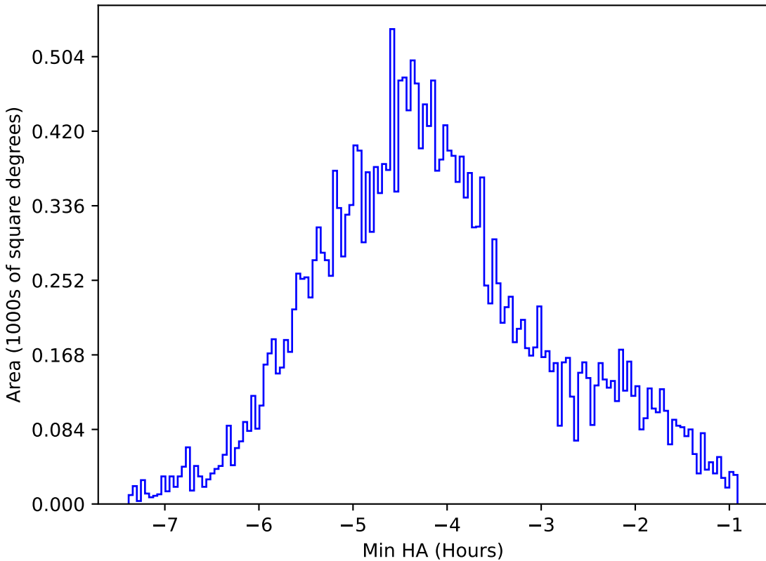
baseline_v3.5_10yrs All sky r band: Min HA
