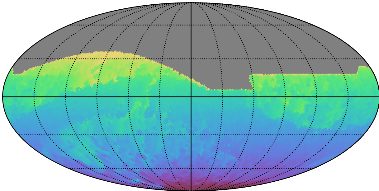
baseline_v3.5_10yrs All sky all bands: Min HA
