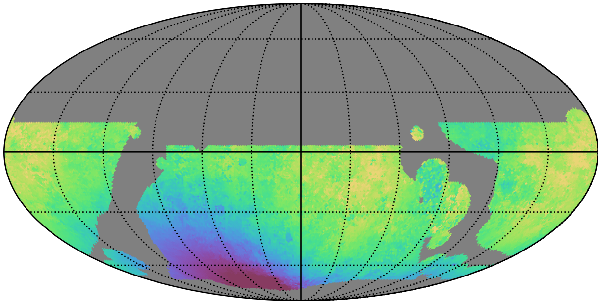
baseline_v3.5_10yrs WFD y band: Median solarElong
