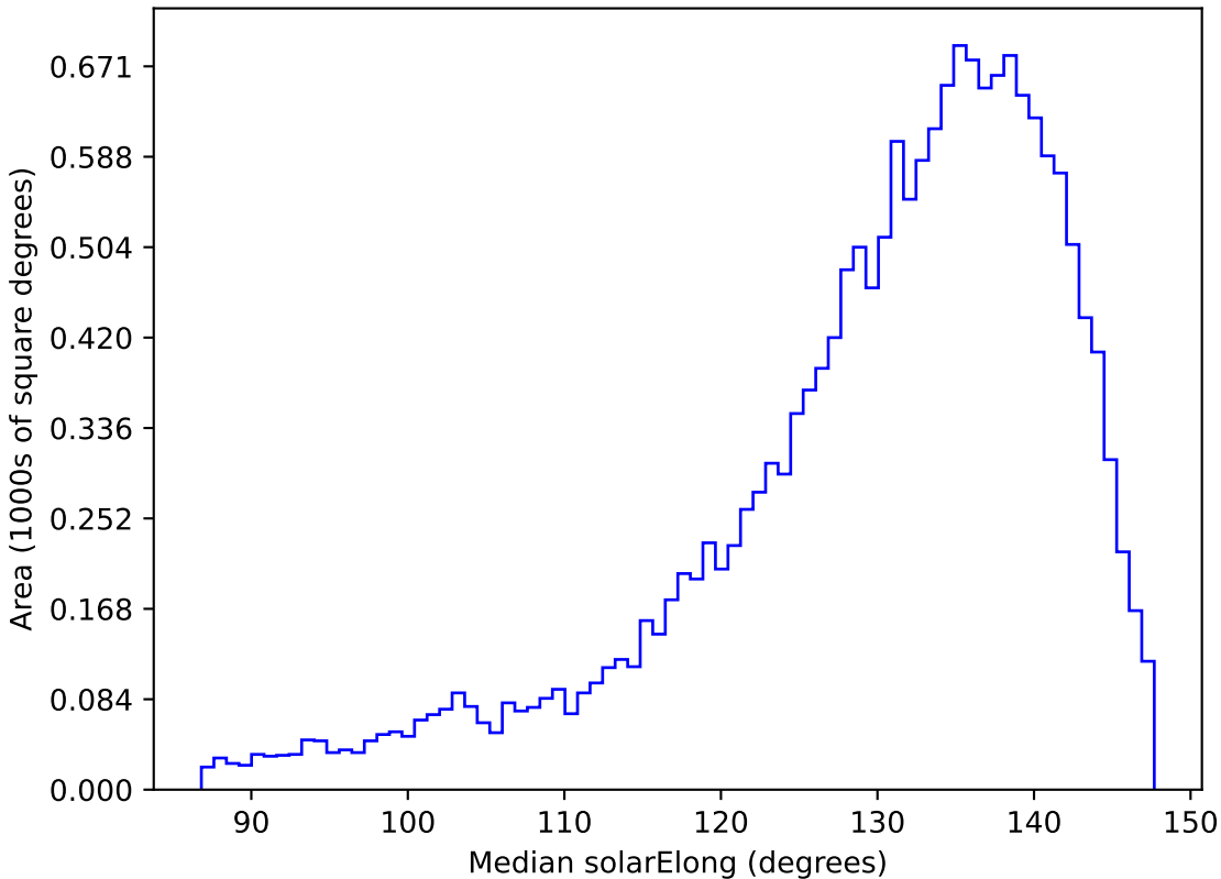
baseline_v3.5_10yrs WFD y band: Median solarElong
