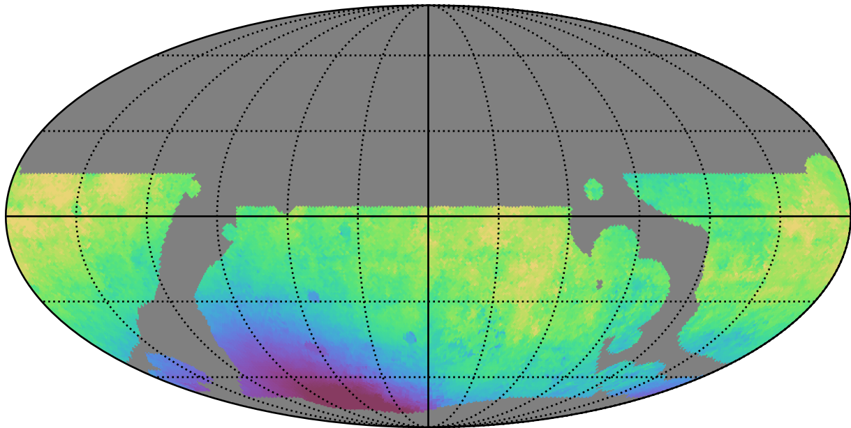
baseline_v3.5_10yrs WFD r band: Median solarElong
