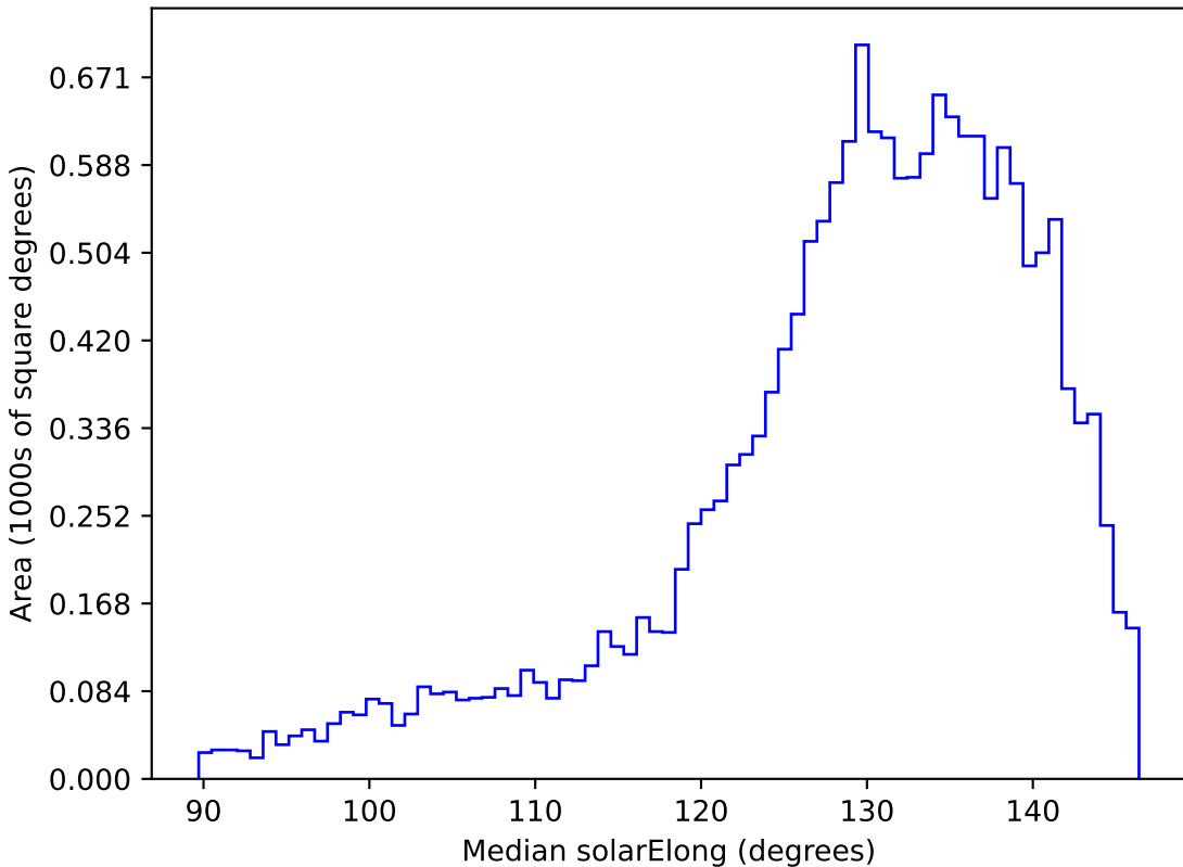
baseline_v3.5_10yrs WFD r band: Median solarElong
