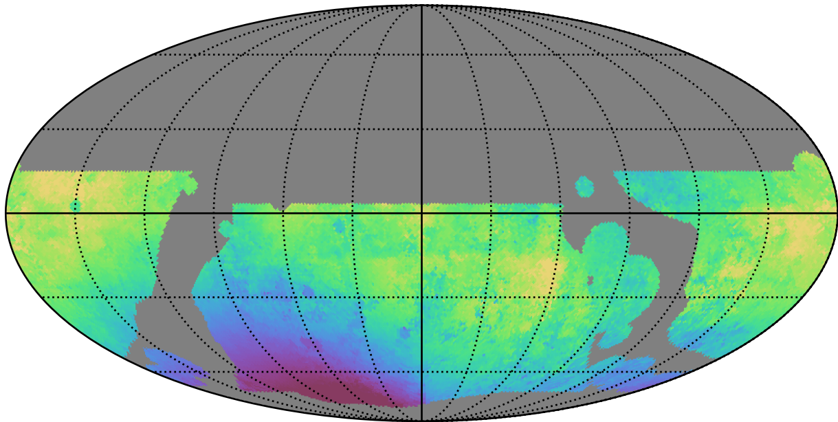
baseline_v3.5_10yrs WFD g band: Median solarElong
