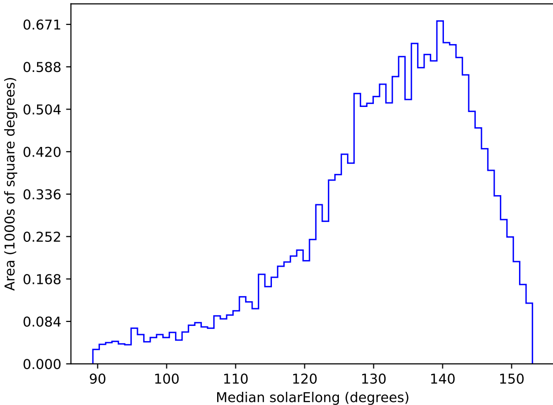
baseline_v3.5_10yrs WFD g band: Median solarElong
