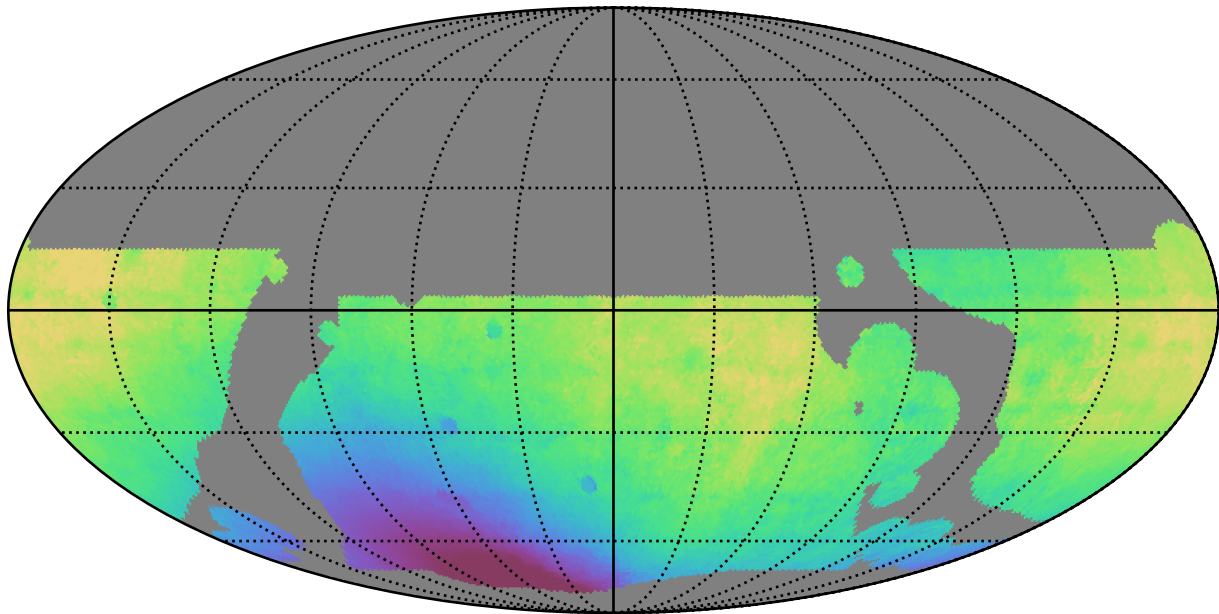
baseline_v3.5_10yrs WFD all bands: Median solarElong
