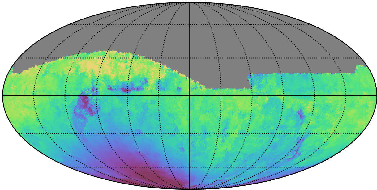
baseline_v3.5_10yrs All sky z band: Median solarElong
