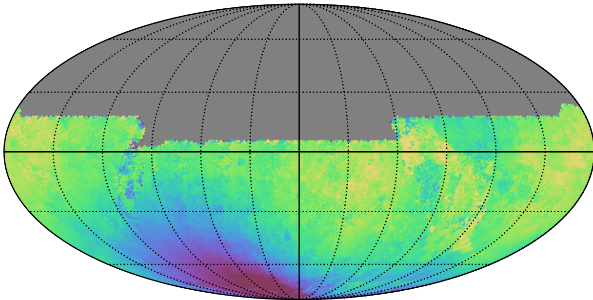
baseline_v3.5_10yrs All sky y band: Median solarElong
