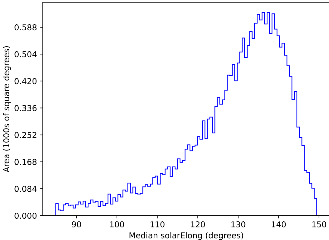
baseline_v3.5_10yrs All sky y band: Median solarElong
