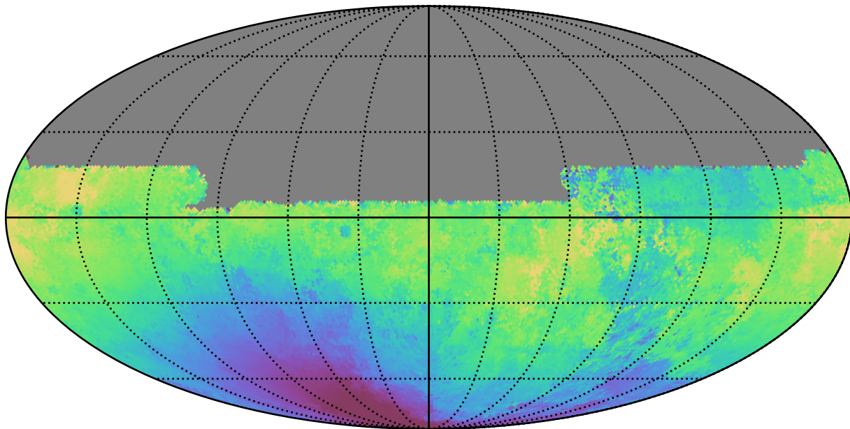
baseline_v3.5_10yrs All sky u band: Median solarElong
