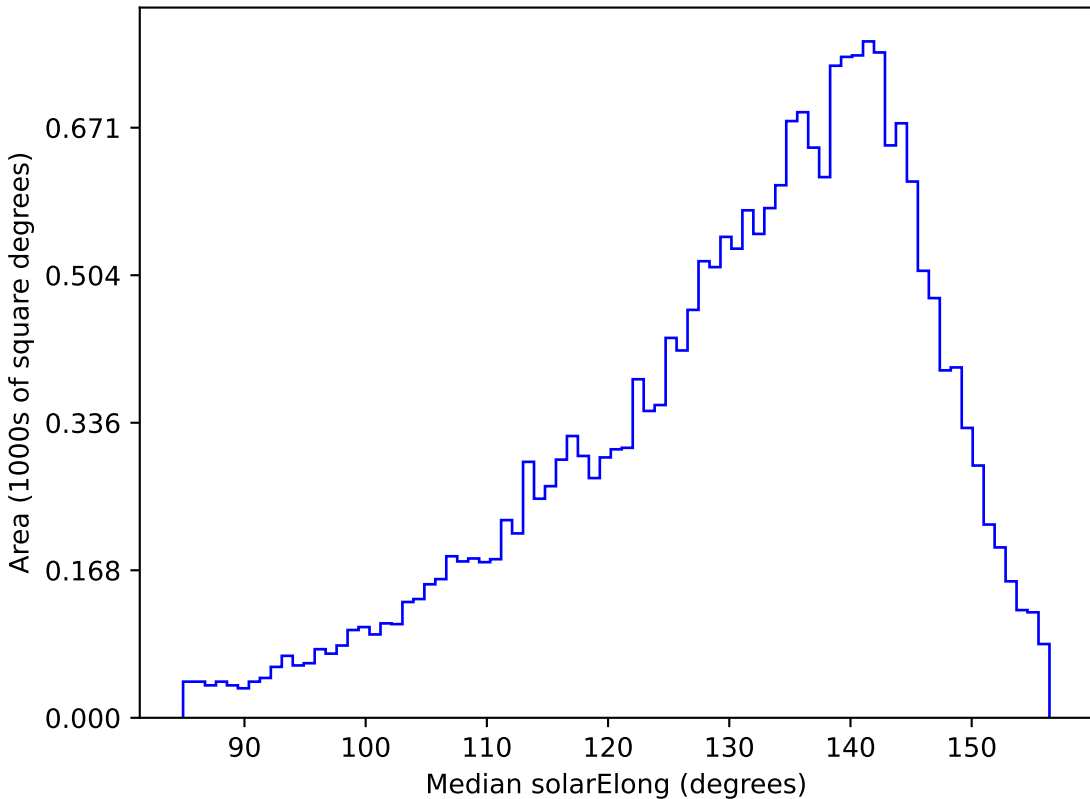
baseline_v3.5_10yrs All sky u band: Median solarElong
